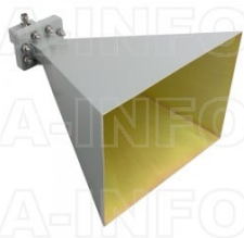
LB-159-20-C-TF Standard Gain Horn Antenna 4.9-7.05GHz 20dB Gain TNC Female
